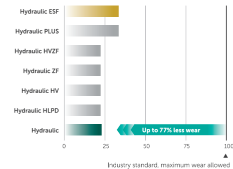
Hydraulic Pump Wear Test Results (test method EATON 35VG25)
